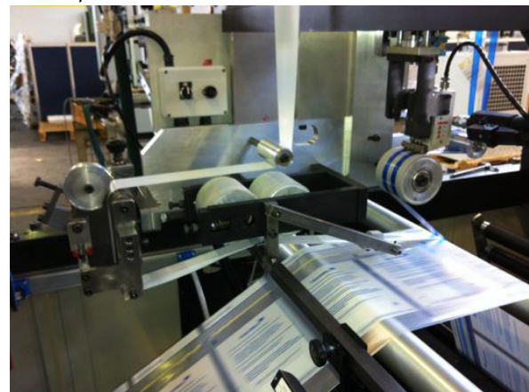
Nastro sicurezza e liner accoppiati con colla / security tape and release liner laminated with hotmelt
